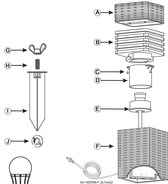
Power LED warm white 12V 6W E27
